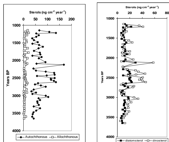
Figure 1: Sterol accumulation rates in core 1.
